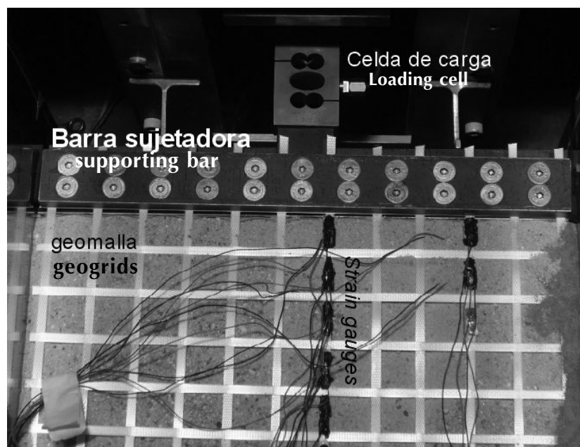
Figura 5. Barra que sujeta las tiras de la geomalla conectada a una celda de carga, strain gauges en la geomalla Figure 5. Bar supporting the geogrids straps connected to a load cell, strain gauges in the geogrids
