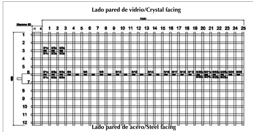
Figura 6. Posición de los strain gauges en la geomalla superior para el caso de ensayo con dos geomallas (geomalla inferior sin strain gauges) Figure 6. Strain gauges arrangement in the upper geogrid, for the case of two-geogrids test (lower geogrids without strain gauges)
