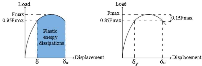
Figure 3. Energy dissipation capacity and load-displacement relationship.
