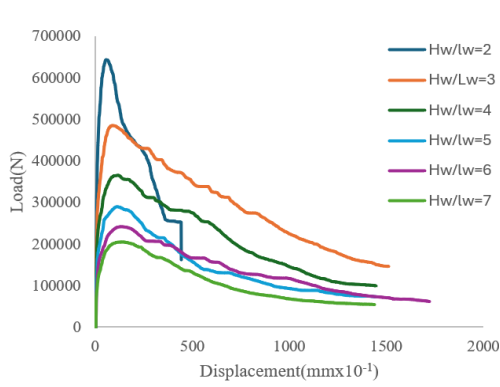
Figure 22. \rho_{sh} = 0.0015 , N/N_o=0.20 load-displacement curves.
