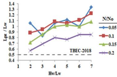
Figure 30. H_w/L_w - L_{pz}/L_w graph for \rho_{sh} = 0.0035 (authors).
